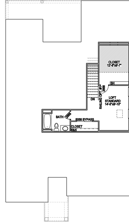
THE YORK (NORTHLAKE) - ELEVATION H OPT. 2ND FLOOR PLAN - 450 S.F.
