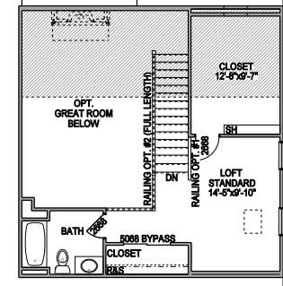
OPT. VAULTED CEILING GREAT ROOM W/ 2ND FLOOR
