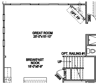
SLAB ON GRADE STAIRS WITH OPT. 2ND FLOOR
