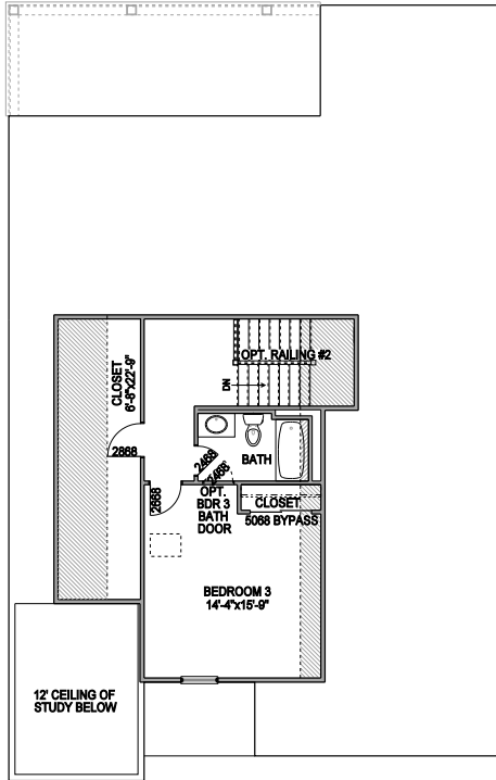
THE CHESTER AT NORTHLAKE OPT. SECOND FLOOR - 560 S.F.
