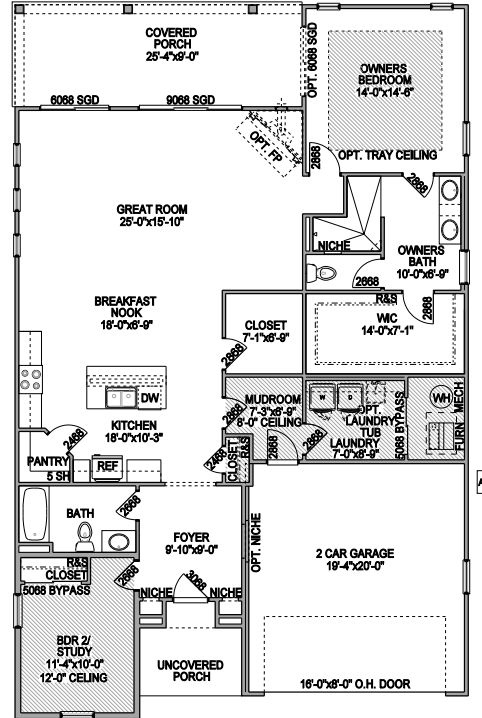
THE CHESTER AT NORTHLAKE STANDARD SLAB ON GRADE FIRST FLOOR - 1,760 S.F. 1,804 S.F. W/ 4' FRONT BUMP
