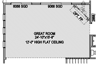
OPT. HIGH FLAT CEILING
