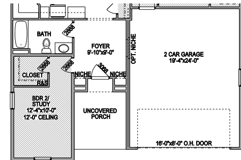
OPT. 4'-0" FRONT BUMP
