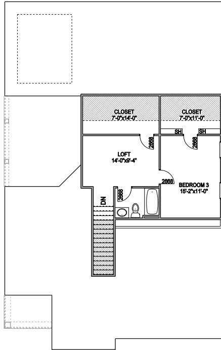
580 S.F. THE HANOVER OPT. 2ND FLOOR
