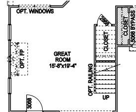
GREAT ROOM W/ OPT. 2ND FLOOR
