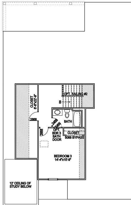
THE CHESTER OPT. SECOND FLOOR - 560 S.F.
