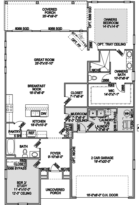
THE CHESTER STANDARD SLAB ON GRADE FIRST FLOOR - 1,760 S.F., 1,804 S.F. W/ 4' FRONT BUMP
