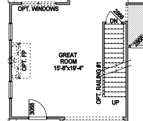
GREAT ROOM W/ OPT. 2ND FLOOR WITH BASEMENT
