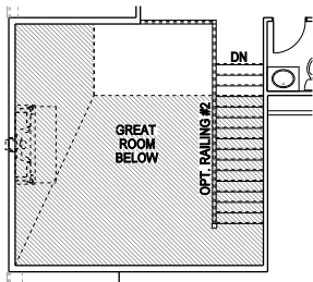
OPT. VAULTED CEILING (ONLY WITH BASEMENT)
