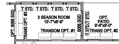
OPT. 3 SEASON ROOM WITH PATIO
