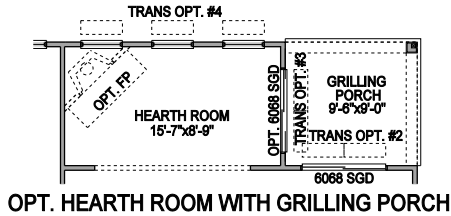
OPT. HEARTH ROOM WITH GRILLING PORCH
