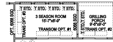
OPT. 3 SEASON ROOM WITH GRILLING PORCH
