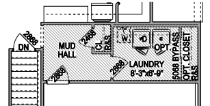
OPT. CLOSET IN LAUNDRY ROOM (ONLY AVAILABLE WITH BASEMENT)
