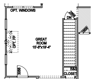
GREAT ROOM W/ OPT. WITH BASEMENT
