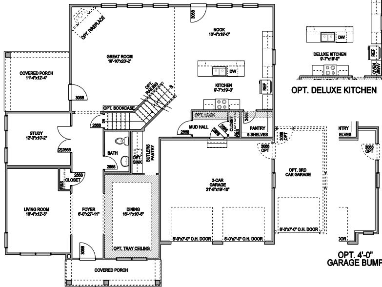
THE HIGHLAND 2 FIRST FLOOR - 1,785 S.F. (2,040 WITH HEARTH ROOM)
