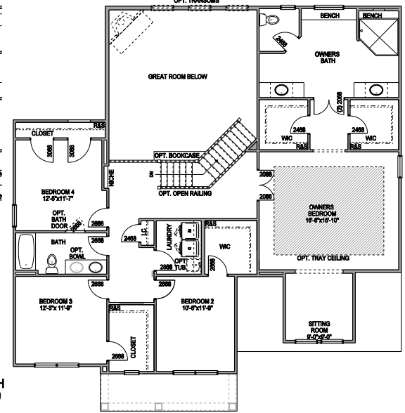
THE HIGHLAND 2 SECOND FLOOR - 1,715 S.F. (2,107 S.F. WITH BONUS ROOM)
