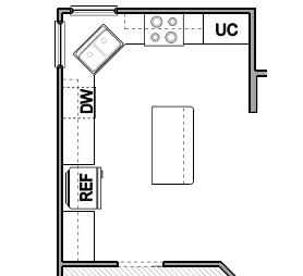
OPT. EXPANDED KITCHEN (ADDS 50 S.F.)
